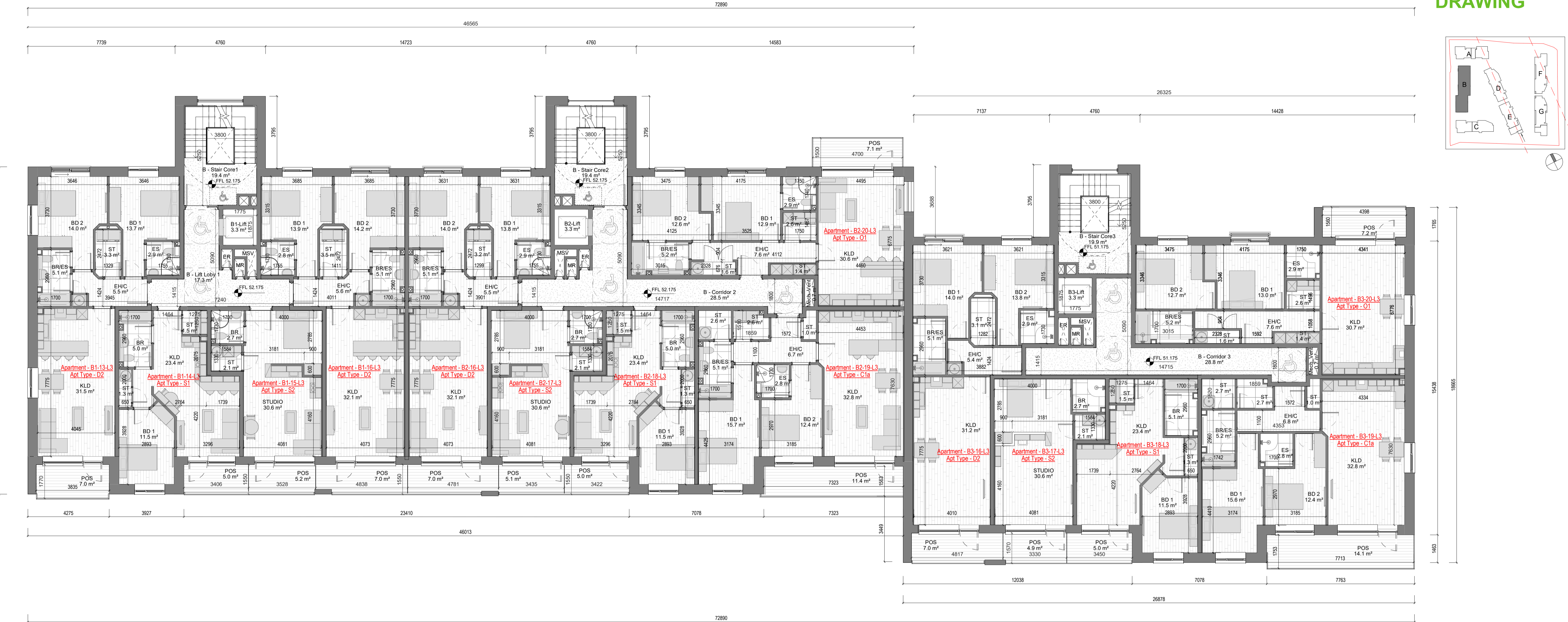
1 GA - Third Floor Plan 1 : 100
